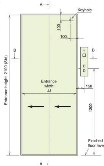
Hoistway entrance
